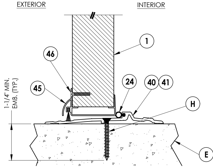
VERTICAL CROSS SECTION Outswing shown
