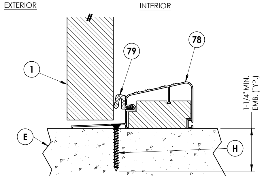
3 VERTICAL CROSS SECTION 5 Outswing shown
